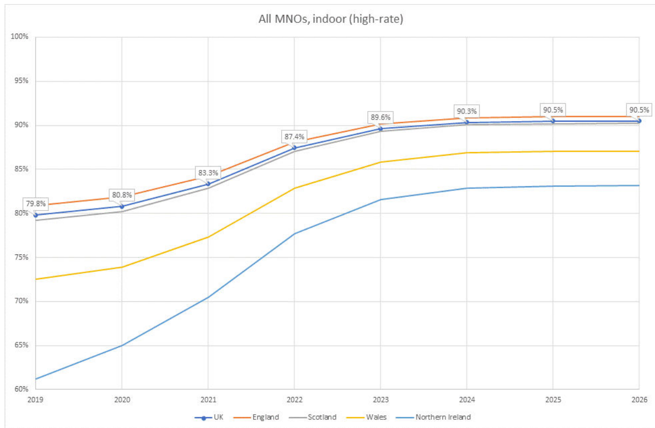
Figure 5.8: Indoor coverage – all MNOs (high-rate)
