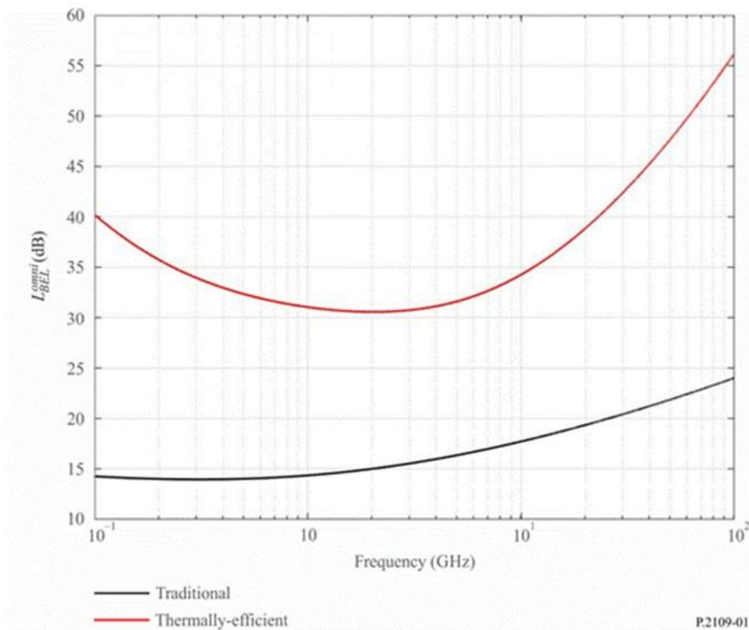
Figure B.2: Median building loss (ITU-R Recommendation P.2109)
