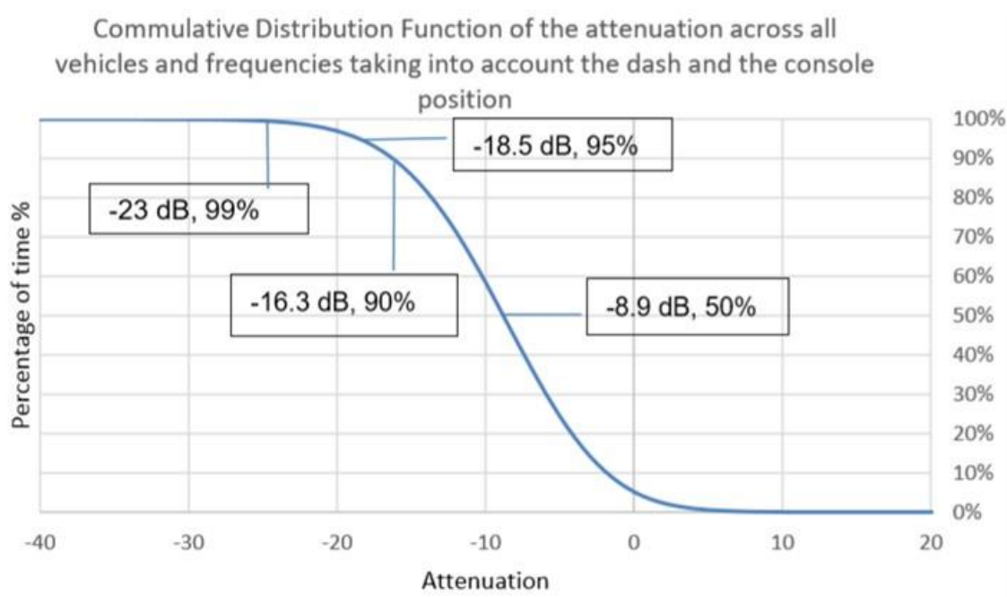
Figure B.4: Vehicle entry losses (LS Telcom report for Ofcom 28 )
